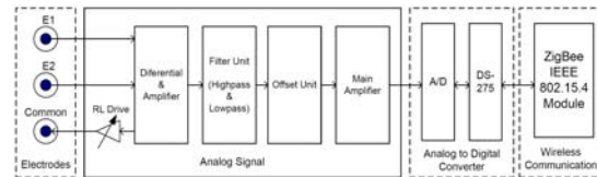
Fig.7:: The design of ECG monitoring via WBBN block diagram.
