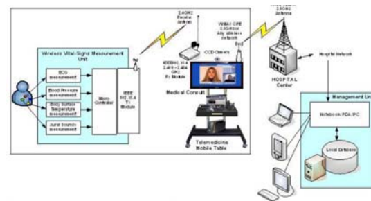
Fig.4:: Structure of telemedicine via WBBN.
