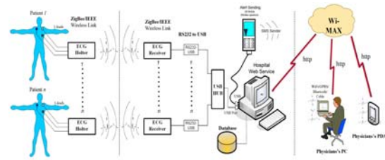
Fig.6:: The structure of the signal processing system in the ECG monitoring.
