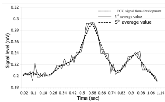
Fig.26:: Shows a comparison of the equation moving average signals in different time periods.
