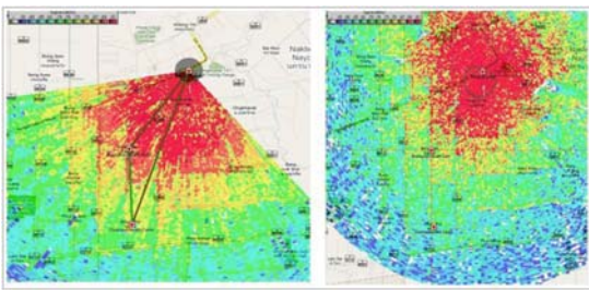
Fig.16:: Radiation pattern of 3-sectors antenna system, the distance between the MSMC to two health sub-district.
